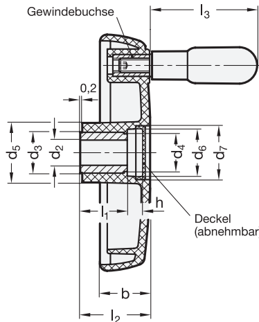
ELESA Original design VDS / VDS-I
