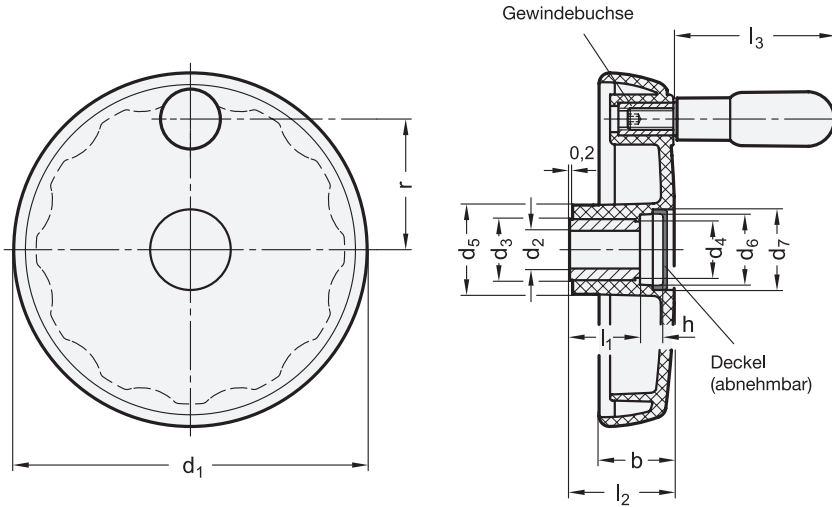
ELESA Original design VDS / VDS+I
